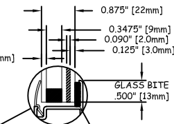
GLAZING DETAIL SCALE 2:1
